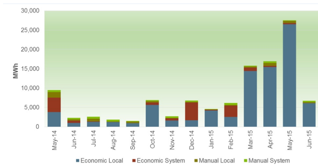
Figure 5. Quantity of Economic vs. Manual Curtailment in the CAISO Markets from May 2014 to May 2015
